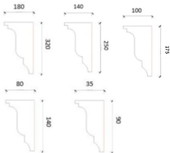
ACE-M25 G1 320x180 - No.14
